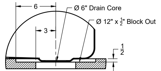
Drain Block-Out
