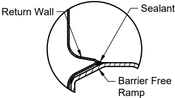
Return Wall Joint
