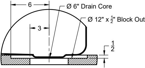
Drain Block-Out
