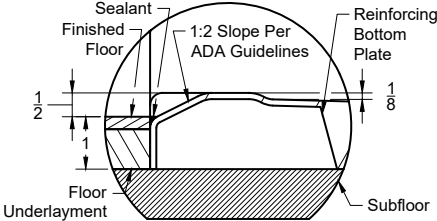
Low-Profile
