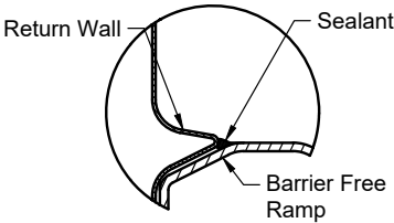
Return Wall Joint
