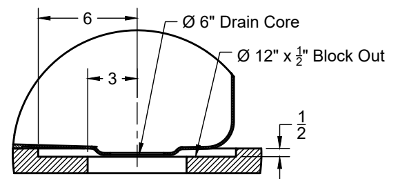
Drain Block-Out
