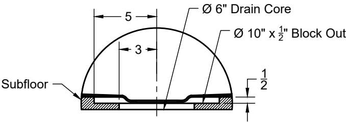
Drain Block-Out
