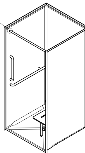
Curtain Rod Detail (See Submittal Sheet Page 3)
