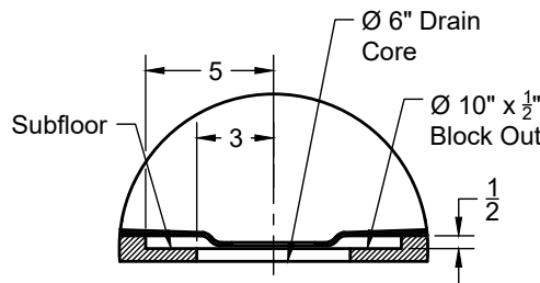
Drain Block-Out
