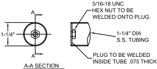
(QNN) NO FLANGE, INTERNAL NUT - DETAIL
