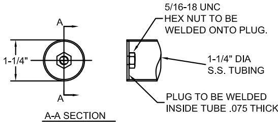
(QNN) NO FLANGE, INTERNAL NUT - DETAIL
