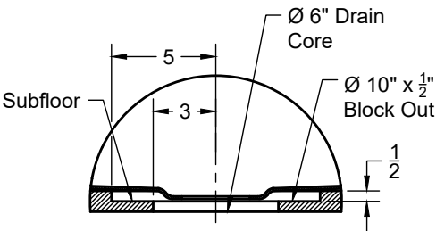
Drain Block-Out
