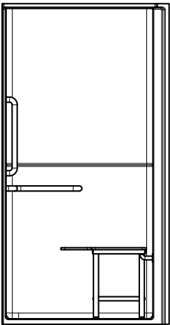
SS3842RFA1-R L-shaped grab bar Seat 18" vertical grab bar
