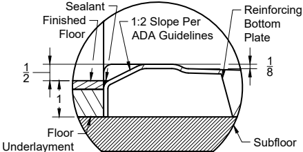
Low-Profile
